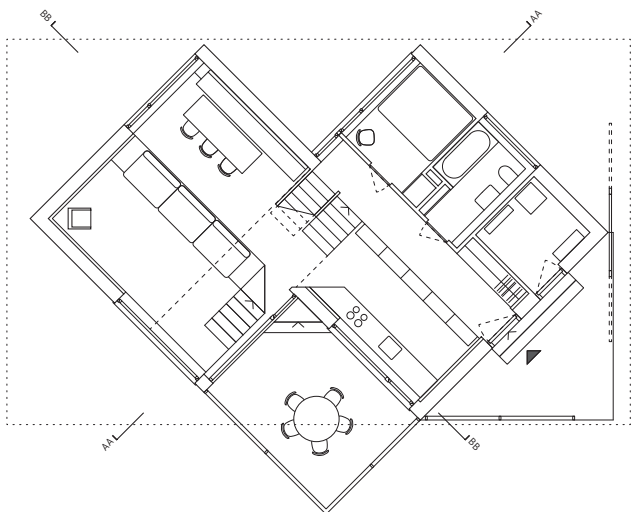
Erdgeschoss/ Ground Floor
