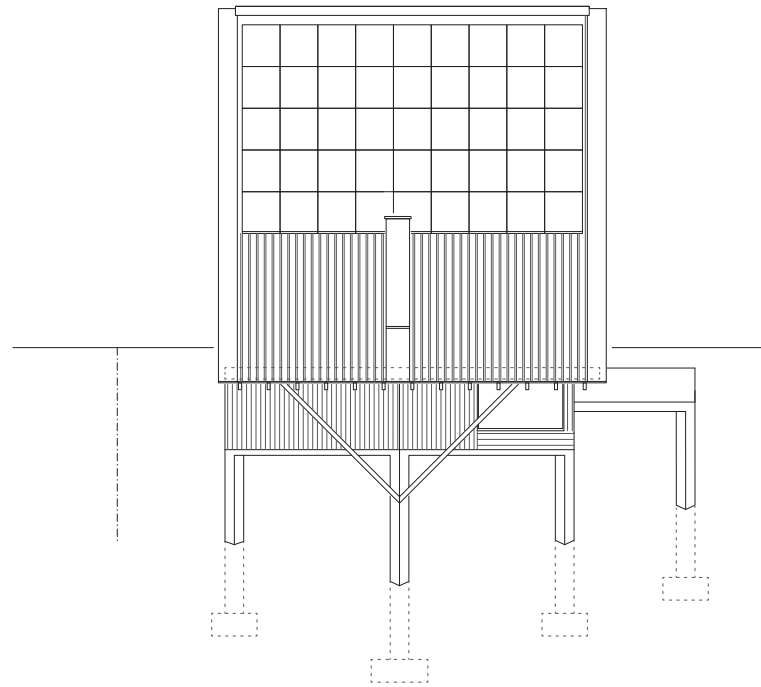
West Elevation
